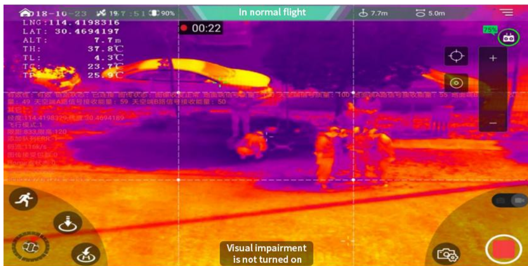
Fig.12 Thermal infrared image of fire alarm, the brighter the color is, the higher the temperature is, which means that an open fire is about to occur and a fire will occur.
