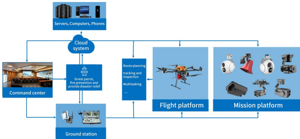
FIG. 2 Functional block diagram of FOREST patrol and fire warning system of GA900 UAV
